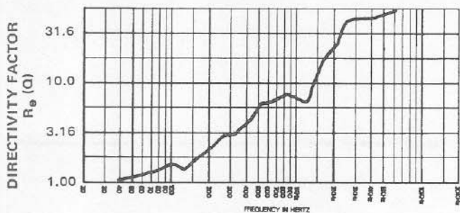
FIGURE 5 TL806/EVM.12L Directivity Factor and Directivity Index vs. Frequency
