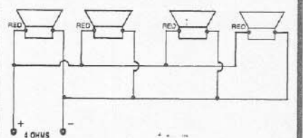
FIGURE 13 Connection of 4 EVM-12L 16 Ohm Speakers in Parallel
