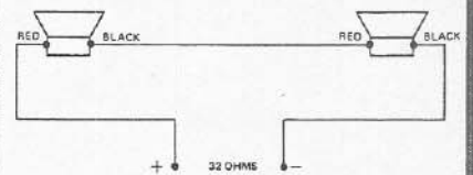
FIGURE 12 Connection of 2 EVM-12L 16 Ohm Speakers in Series
