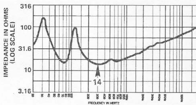
FIGURE 8 TL806/EVM.12L Input Impedance vs. Frequency
