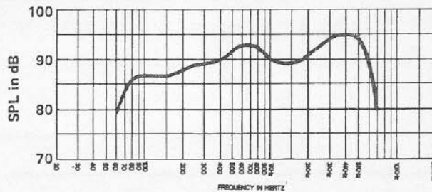
FIGURE 2 - TL806/EVM.12L Frequency Response (Swept 1/3-Octave Band Pink Noise, 4 V at 10 ft. on Axis, Half-Space Environment)
